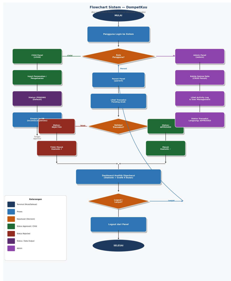
Gambar 2. Flowchart Sistem DometKuu — Alur Login Multi-Panel & Approval Workflow
